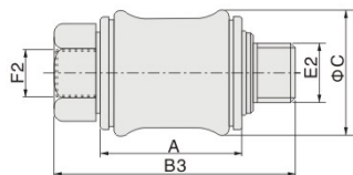
外内牙型(MF)/Male and female thread(MF)
